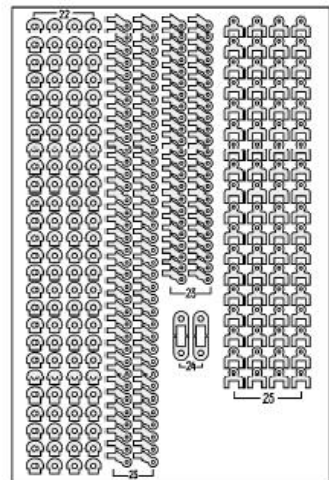
3mm non-laminated
