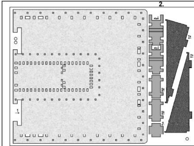
6mm laminated
